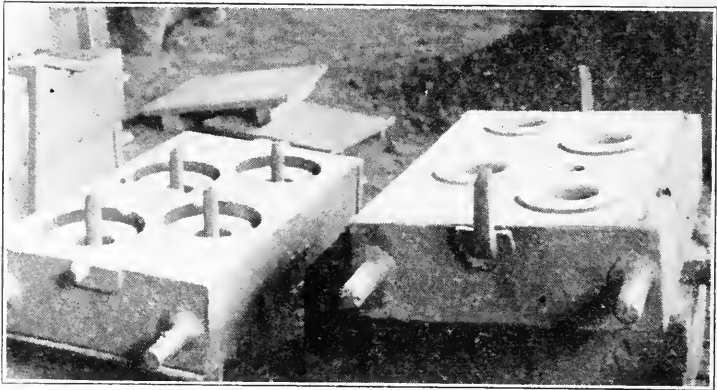
FIG. 534. VERTICAL DRY-SAND CORES.
